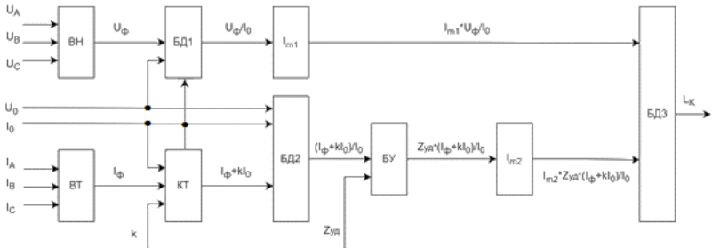
Fig. 1. Block diagram of the device for determining the location of damage according to (1)
